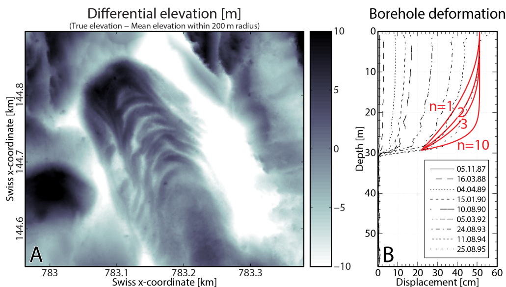
Figure 1: A) Differential DEM of Murtèl rockglacier [Frehner et al., 2015]. B) Time-lapse borehole deformation data [Arenson et al., 2002]. Red: theoretical flow geometries using different non-linear viscous flow laws ( n = 1 : linear viscous; n = 10 : strongly non-linear).
